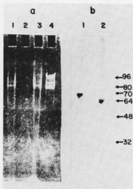
Fig. 4. Agarose gel electrophoresis of viral DNA and protein. (a) The viral DNA was electrophoresed on a 0.8% agarose gel untreated (lane 1), treated with 2 mg/mL pancreatic deoxyribonuclease for 30 min at 37°C (lane 2), and treated with 2 mg/mL T1 ribonuclease for 30 min at 37°C (lane 3). An EcoRI restriction endonuclease digest of bacteriophage \lambda DNA was run in lane 4 for size determination. (b) The viral protein was electrophoresed on 5% SDS polyacrylamide disc gels. Untreated virus was run in lane 1 after boiling SDS extraction and virus treated with 50 \mu g/mL trypsin for 2 h at 37°C was run in lane 2 after boiling SDS extraction. The numbers alongside indicate the location of molecular weight marker proteins with sizes in thousands. The gels were stained with Coomassie brilliant blue.
